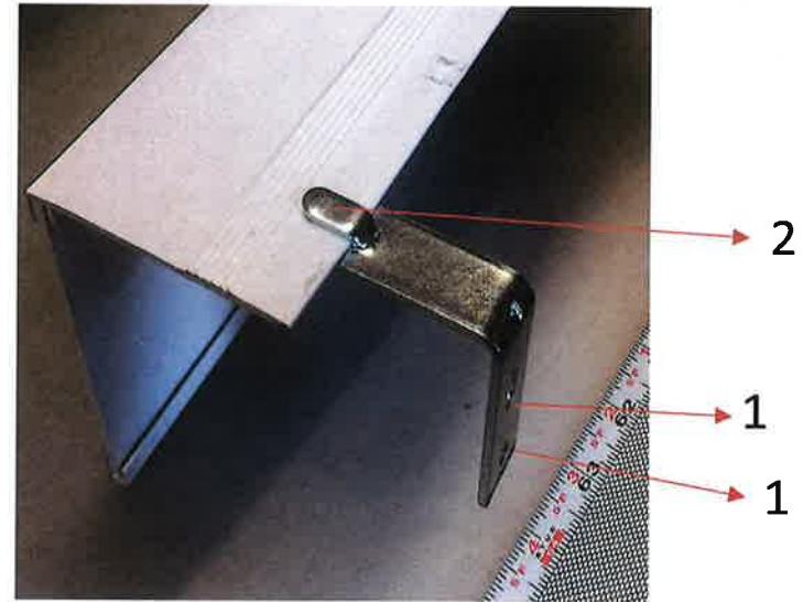
Wall Mount
